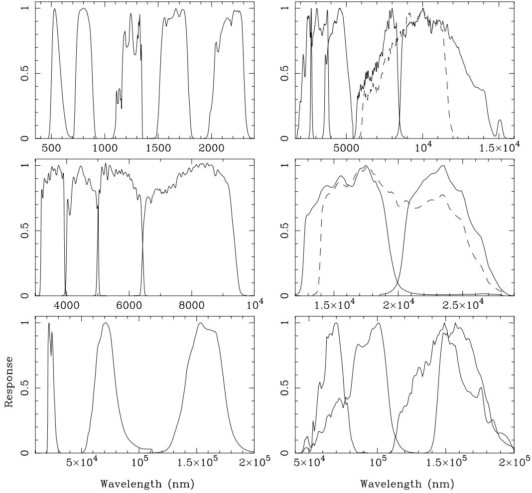
Fig. 2. Filter curves adopted: Bessell VI , 2MASS JHK (left top), Spitzer-IRAC (left middle), Spitzer-MIPS (left bottom), ASTRO-F IRC and MIR-S (right top), ASTRO-F MIR-L (right middle), and ASTRO-F FIS (right bottom).
