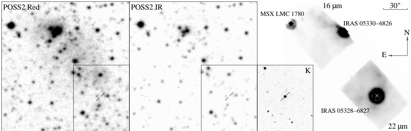
Figure 2. A POSS2 red image (left), which includes H\alpha emission, shows the H\text{ II} region LHA 120-N 148 A and a compact cluster embedded in it. The cluster stands out better on the POSS2 IR image (centre). IRAS 05328–6827 only becomes visible at wavelengths beyond \sim 1\ \mu\text{m} and is one of the brighter stars in the MSSSO K -band image. The IRS red peak-up image (right) shows an intense source at 22\ \mu\text{m} . Coincidentally, the blue peak-up image at 16\ \mu\text{m} includes the cluster, IRAS 05330–6826, and a stellar mid-IR source, MSX LMC 1780.
